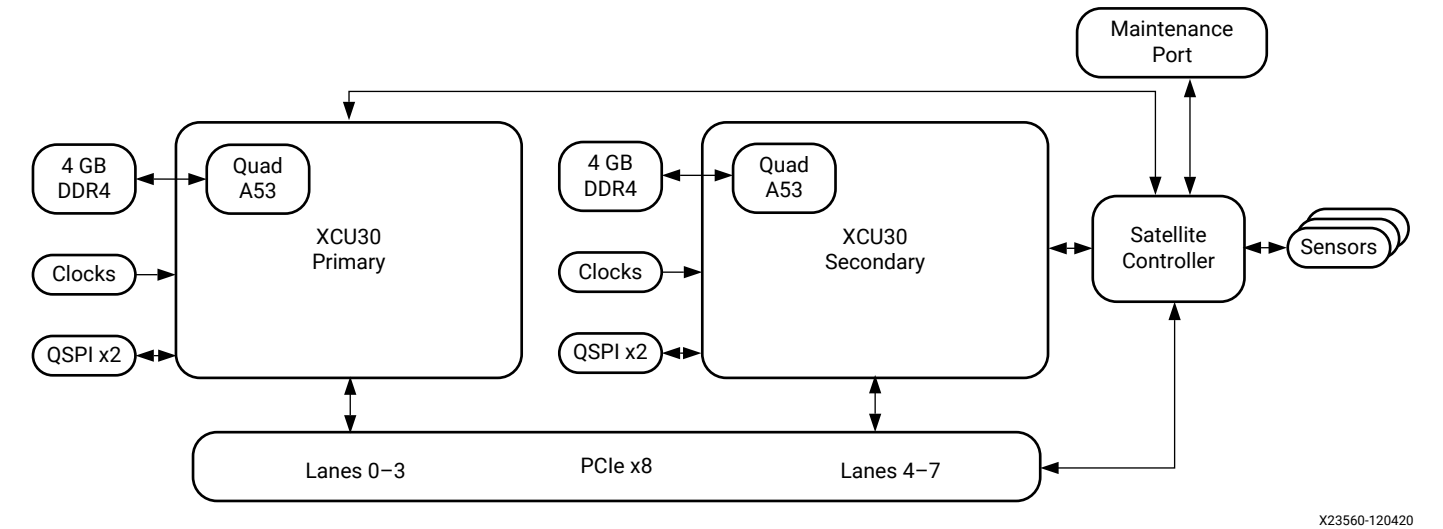
Figure 2: U30 Block Diagram
